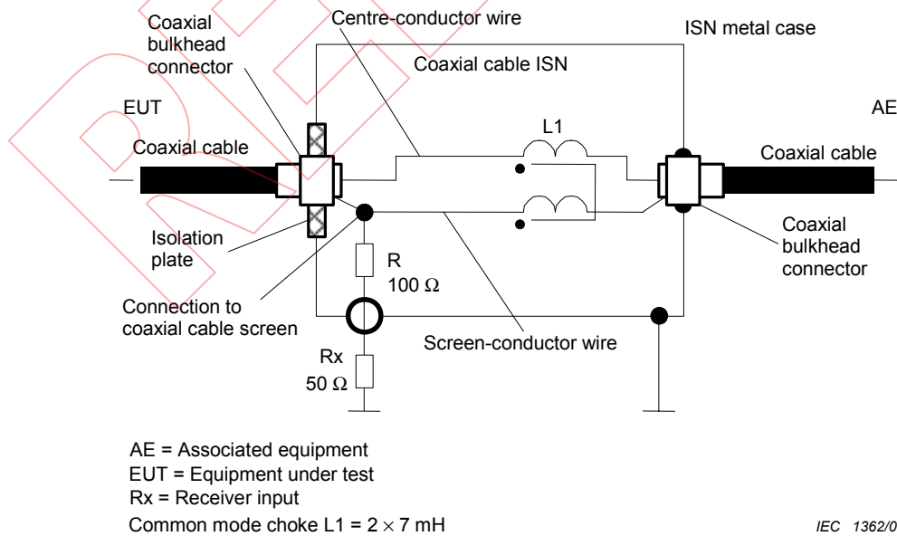
Figure D.7 – ISN for use with four unshielded balanced pairs
